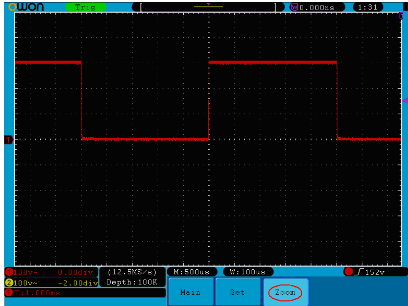
Figure 5-15 Zoom Window
