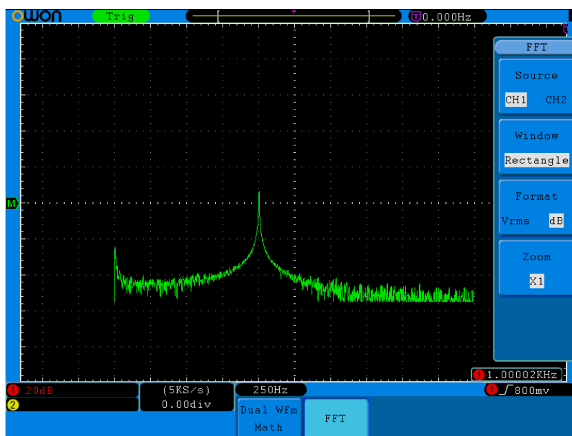
Figure 5-10 Rectangle window
