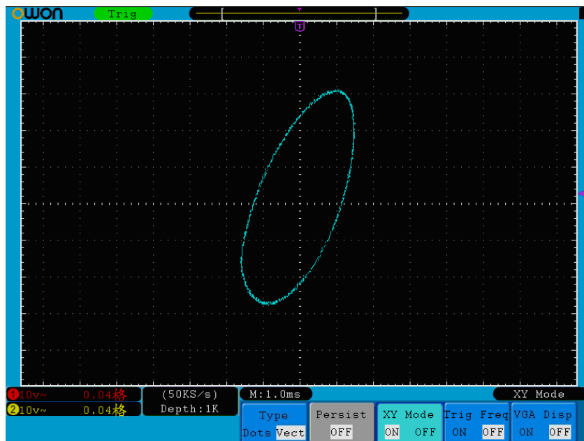
Figure 5-32 XY Display Mode
